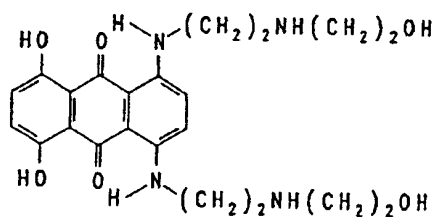
Mitoxantrone
